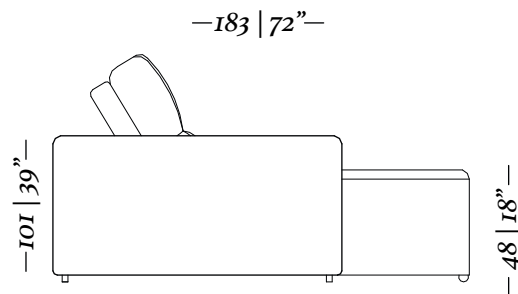
Chaise retr[atil/ Retractable chaise 1 Braço/ Arm 25cm Ass. 110cm
