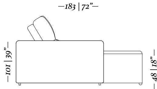
Chaise retr[atil/ Retractable chaise 1 Braço/ Arm 25cm Ass. 90cm
