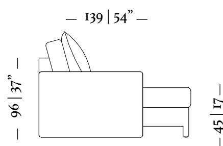
Chaise retrátil/ Retractable chaise 01 Braço/ Arm 20cm Ass. 110 132 x 98 x 96cm
